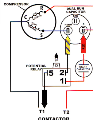
DUAL RUN CAPACITOR
