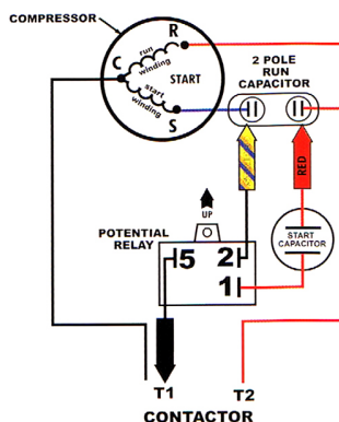
2 POLE RUN CAPACITOR
